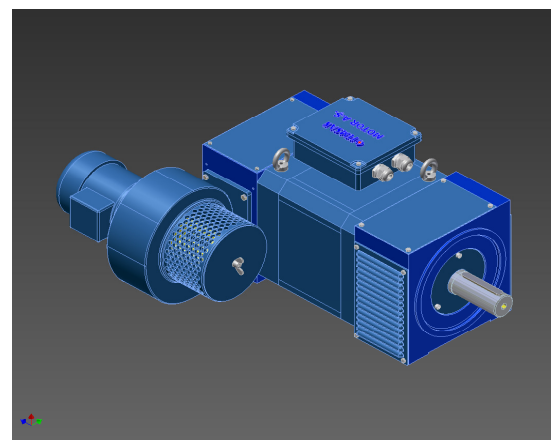
Terminal Box at top Blower NDE side, left
