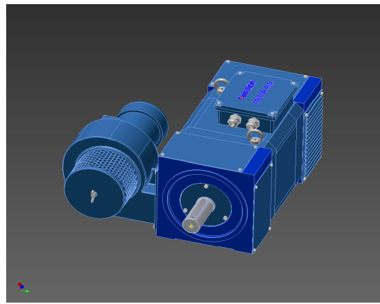
Terminal Box at top Blower DE side, left
