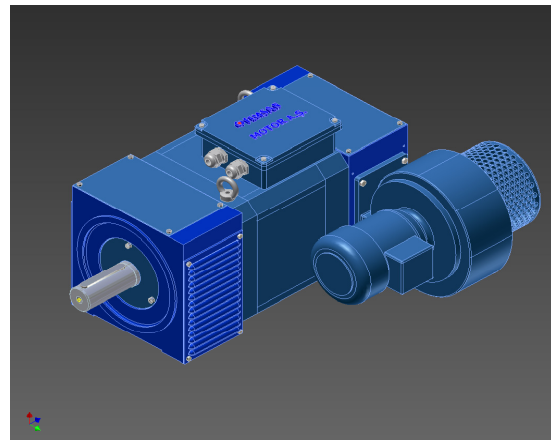
Terminal Box at top Blower NDE side, right
