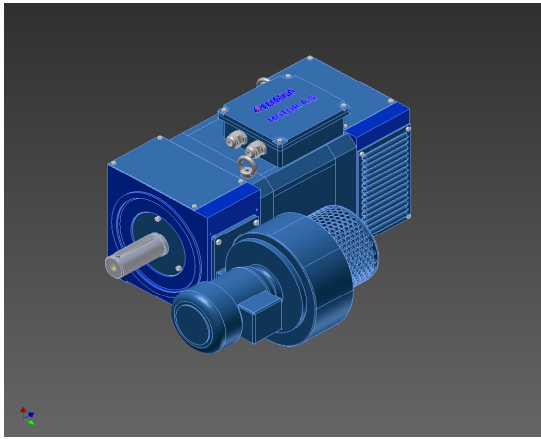
Terminal Box at top Blower DE side, right
